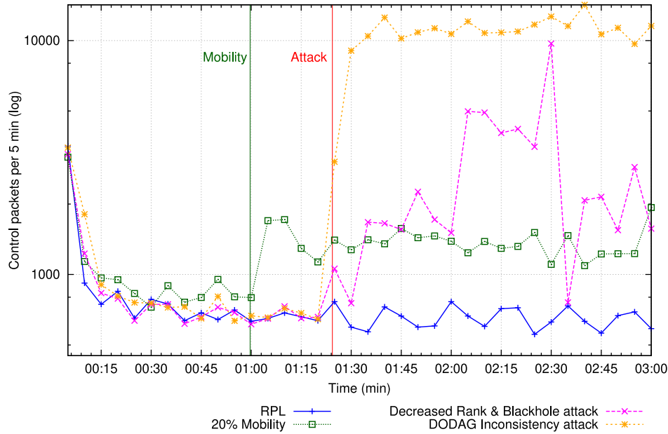
Fig. 5 – Control overhead under attack and mobility over time.
