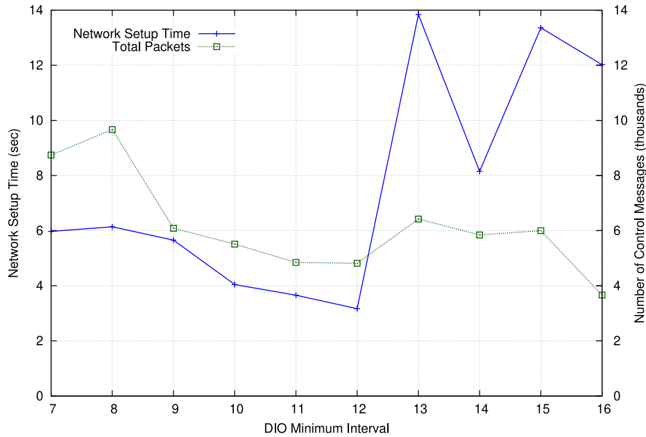
Fig. 3 – The network setup time and control overhead in respect to the DIO I_{\min} .
