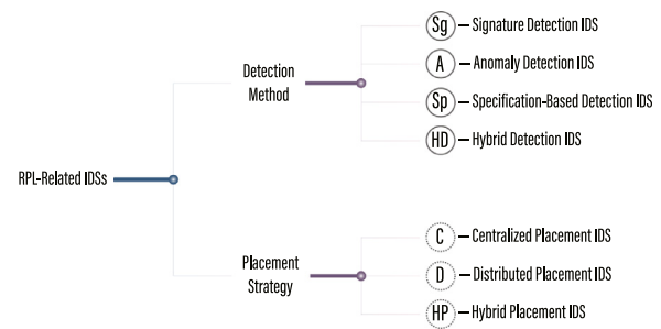
Fig. 7 – Classification of IDSs in respect to their detection method and their placement strategy.
