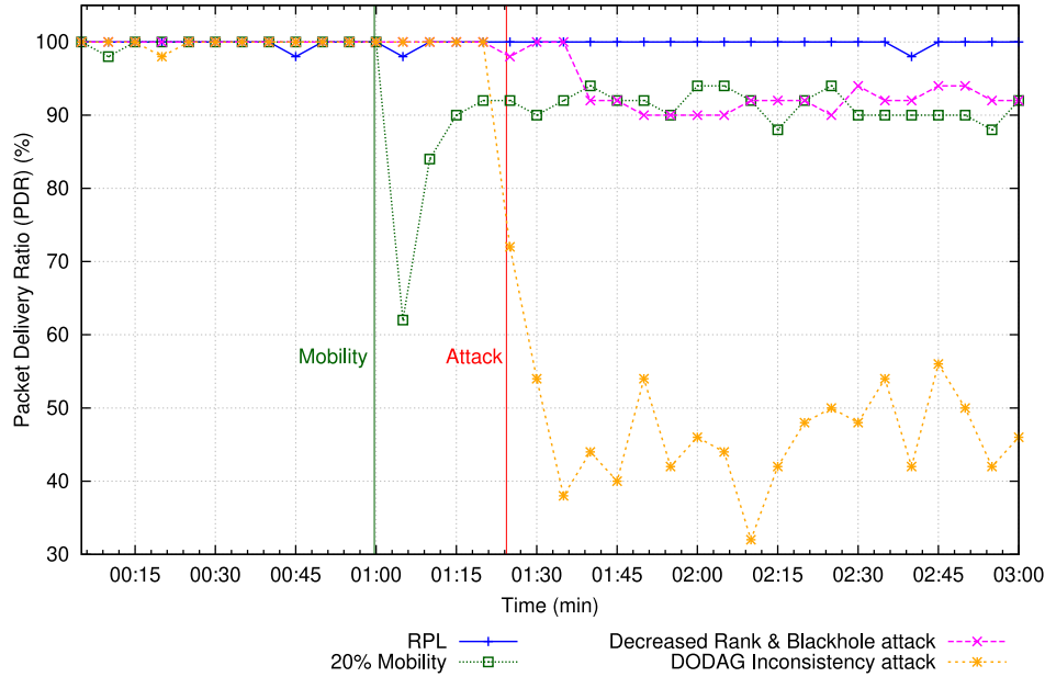
Fig. 6 – PDR under attack and mobility over time.
