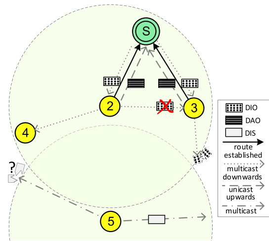
Fig. 2 – DODAG construction.
