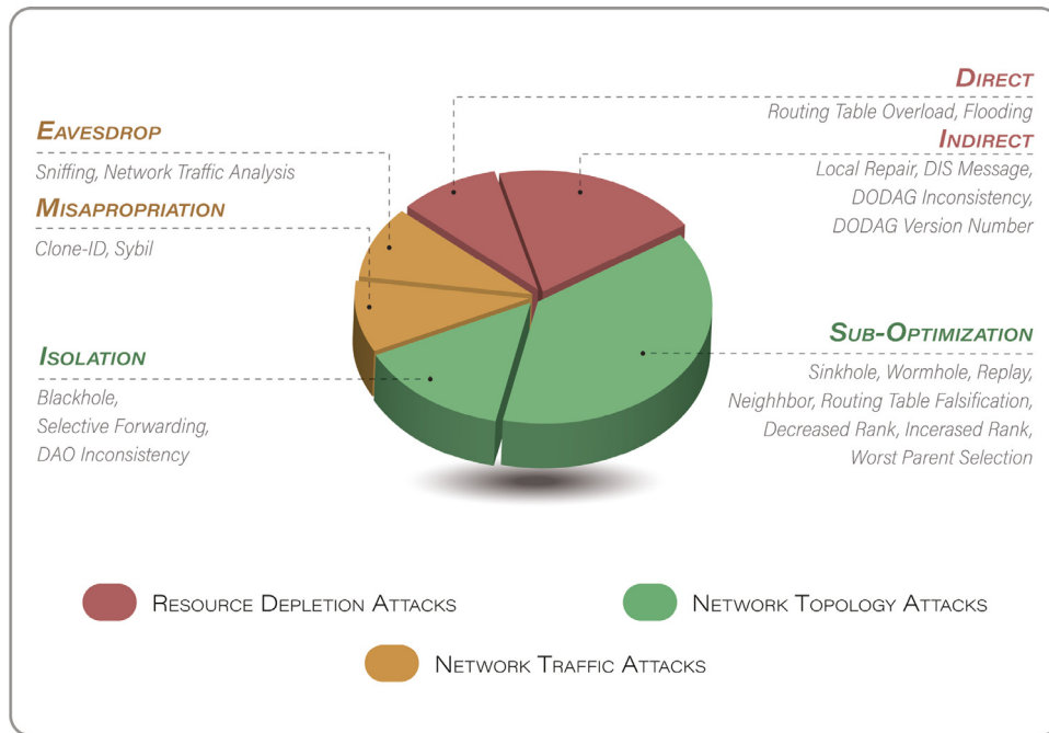
Fig. 4 – Classification of RPL attacks.
